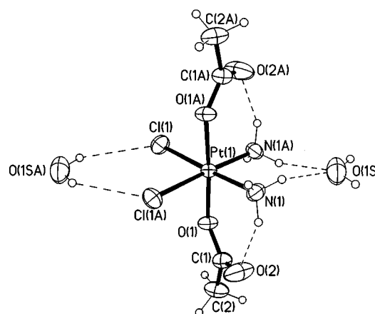
Fig. 1 Molecular structure of complex 1 showing intra- and inter-molecular hydrogen bonds.
